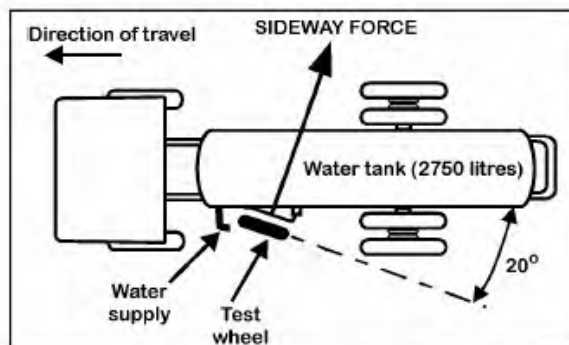
Diagrammatic Layout of SCRIM
